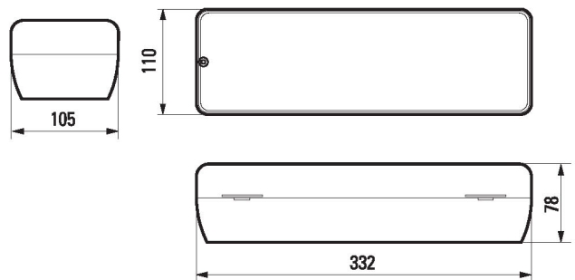
Single sided Dimensions [mm]
